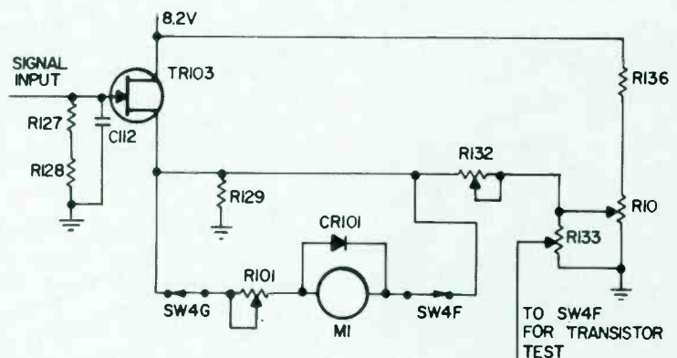
Fig. 2 An FET is used to obtain a very-high input impedance, and the drain-to-source resistance is used as one leg of a bridge which drives the meter for all tube-testing functions. (Courtesy of Sencore)
