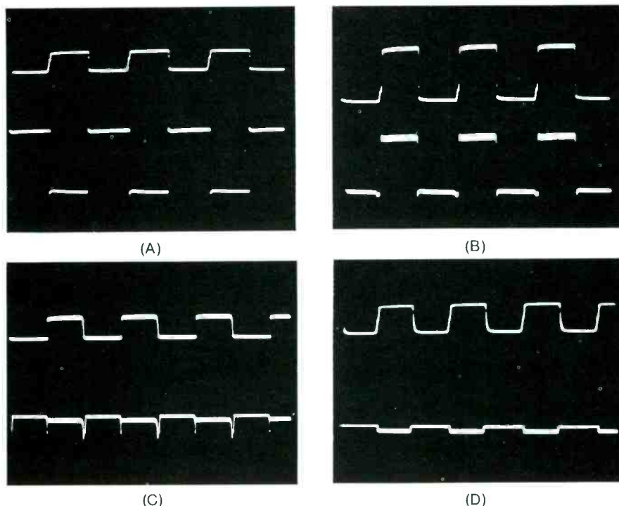
Fig. 5 These are the waveforms and voltages obtained by operation of the six lead-switching pushbuttons. (A) A small NPN silicon transistor was connected yellow to base, green to emitter, and red to collector; then the PNP Gain test was selected and button #1 was pushed. This was the correct (or standard) wiring which produced a "good" reading and a Cricket audio tone. The waveform at top is the base signal, a 2 V p-p 2800 Hz square wave; the DC reading was -.41, evidently from self-rectification of the signal, for without a transistor it was -.15V. Bottom waveform is the 180° 6V p-p collector signal (+2.65 with transistor, +5V without). (B) Same conditions as (A), except button #4 was pushed. Top waveform is the 6V p-p -3.04 V (-5V without transistor) signal at the base. Waveform at bottom is 4V p-p non-inverted one at the red wire, now connected to the emitter. DC voltage is -2.66 with transistor and -5V without. This is the false connection, which also produced a good gain reading and Cricket tone. (C) Button #3 gave no reading. Top trace is the signal at the yellow wire (now the emitter), while the trace at the bottom consists of negative-going edges of the input square waves (now connected to the base). Button #5 also gave no reading. The waveforms were the same except the one at the red wire (now collector) consisted of positive-going pulses. Buttons #2 and #6 gave no waveforms. (D) These are the same conditions as (A), except a 100K resistor was placed in series with the yellow wire (base). Waveform at the base was normal (top trace), but the square waves at the collector were very weak (trace at the bottom). However, the meter showed a normal reading and a normal Cricket tone was heard. When the button #4 for false connection was pressed, the meter read "?", the Cricket tone was weak, and the scope waveform showed very little amplitude of output signal.
