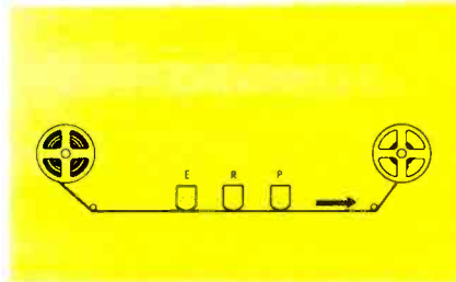
Fig. 5 The tape moves past the erase head, record head, and the playback head in that order. Some machines use one head for both record and playback functions.
