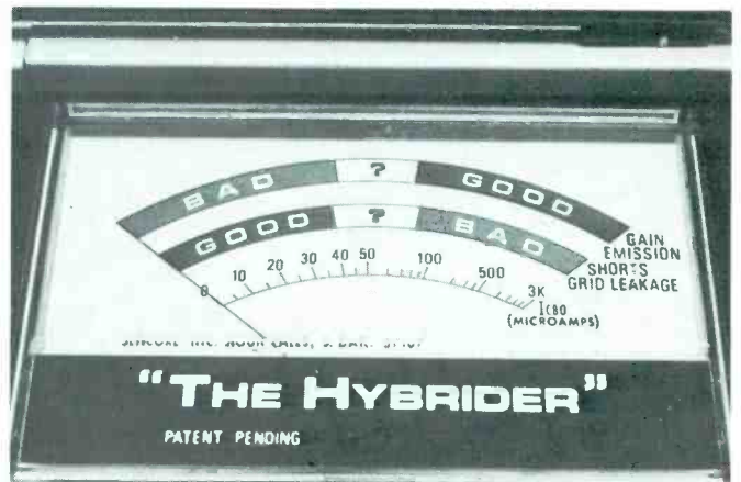
Fig. 4 Three scales are on the meter face. Top one is the good-bad scale for tube emission or transistor gain, center scale is for tube shorts and grid leakage, and the one at the bottom shows transistor leakage in microamperes.
