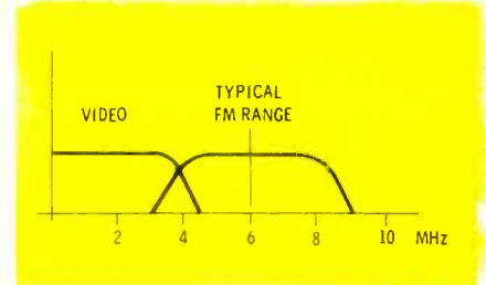
Fig. 6 Frequency modulating a carrier is an excellent way of reducing the 150,000-to-1 ratio of video frequencies to only 2-to-1.
