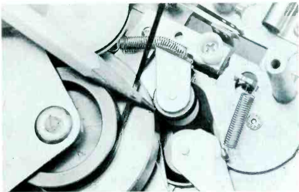
Step 15. Rewind and Fast Forward usually are driven from the same flywheel idler. The entire fast-forward drive train, plus an extra idler, comes into use when you press the Rewind button. The rewind idler, the added one, presses against both fast-forward idler and supply spindle, spinning the spindle rapidly in reverse. Usually, you'll find no torque adjustment here. If rewind becomes erratic or too slow, you hunt for weak or unhooked springs or binding idlers.
