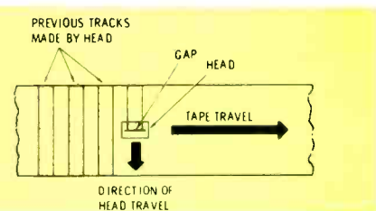
Fig. 7 One way of obtaining a high head-to-tape speed at a slow tape speed is to rotate the head in a circle perpendicular to the length of tape, making tracks across the width. However, more than one head must be used to avoid gaps.
