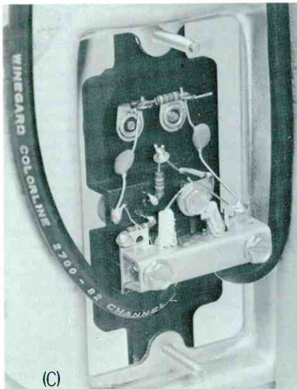
Fig. 1 These are three examples of poor workmanship in the wiring of an MATV tapoff, plus one example of good practice. (A) This can be your standard of correct wiring. Both center conductors are under the screw head and the excess has been cut. Sections of the shields have been twisted and located under the ground clamp. The amount of stripping and the location of the cables are good. (B) One of the center conductors is not under the screw head, and the
