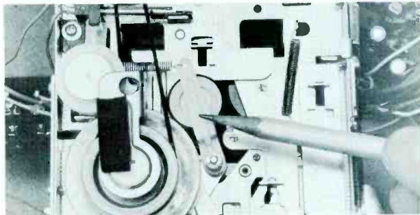
Step 14. When you press the Fast-Forward button, at least three mechanical actions must occur: (1) the power switch closes, (2) the spindle brakes release, and (3) the fast-forward drive train engages. Underneath, a rubber-rim idler presses against the flywheel to initiate fast-drive motion. A pulley on the idler shaft drives a rubber belt that turns the fast-forward idler. The idler presses against the takeup spindle, driving it directly. If either of the idlers get sloppy or bind, or if tension springs get weak, tape takeup might become slow or erratic. Few cassette machines have an adjustment for fast-forward torque. Cleaning, and replacement of faulty parts, are your chief remedies.
