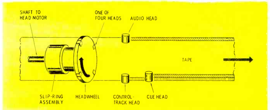
Fig. 8 Four heads equally spaced around a wheel rotating inside a curved wide tape provide overlap between tracks of the heads.
