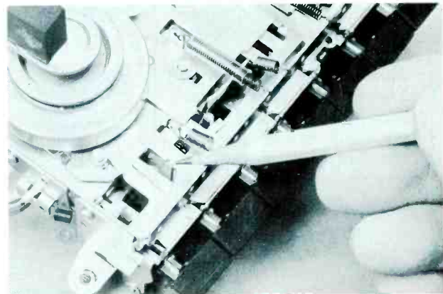
Step 16. Normally, the Stop button has only one job. It slides the latch-plate to release whichever button is depressed. Springs do the job of returning assemblies to their resting or nonoperating positions.
