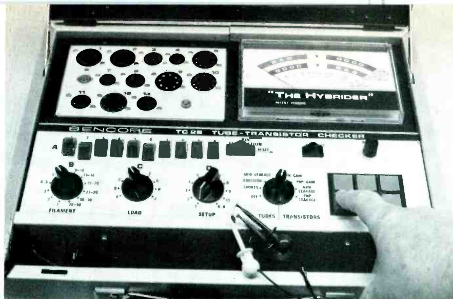
Fig. 7 Six pushbuttons at the lower right corner of the TC28 permit correct connection of transistor and test clips.
