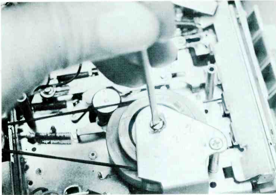
Step 13. Some machines have an adjustment to eliminate flywheel play. You simply adjust the screw (or bracket, on some models) for minimum vertical movement. Don't get it so tight the flywheel can't "coast" well when you spin it (keep fingers off the drive surface).
