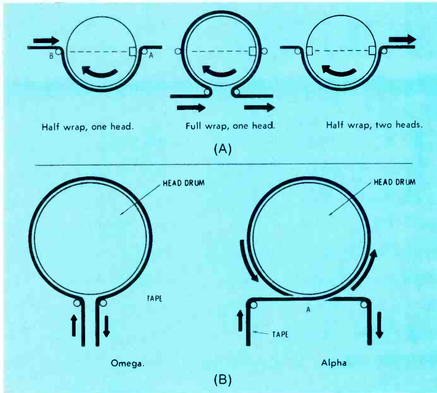
Fig. 11 Various models have different number of heads and types of tape wraps. (A) Two heads or one can be used with a half wrap of tape, or a full wrap might be used with a single head. (B) There are two kinds of full-wrap paths. The alpha more than encircles the drum, permitting less loss of signal between tracks, while the omega does not complete the circle.
