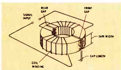
Fig. 2 Audio recording heads are made with two halves of laminated-iron or powdered-iron cores, and one winding on each half. This is essentially a toroid, and is not sensitive to picking up hum from external fields.
