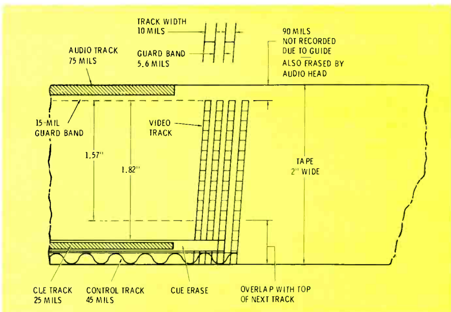
Fig. 9 This is the arrangement of the three longitudinal tracks and the nearly-perpendicular video tracks of a quad-head recorder.
