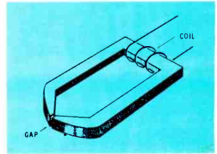
Fig. 12 Video heads have only one narrow gap in the powdered-iron core and just a few turns of wire.
