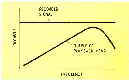
Fig. 4 A tape that has been recorded with constant current (equal magnetic fields for all frequencies) will have a roll-off of both high and low frequencies (unless compensated) when played.
