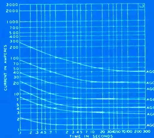
Time-current characteristics of BUSS® fast-acting fuses
