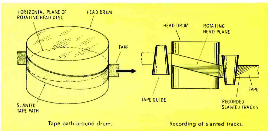
Fig. 10 Principle of the helical (or slant-track) video recorder is to obtain a track long enough to record satisfactorily one vertical field by wrapping a half or full turn of tape at an angle around a motionless drum and using a rotating head operating through a slot in the drum. The resulting tracks are long, and are slanted relative to the tape.
