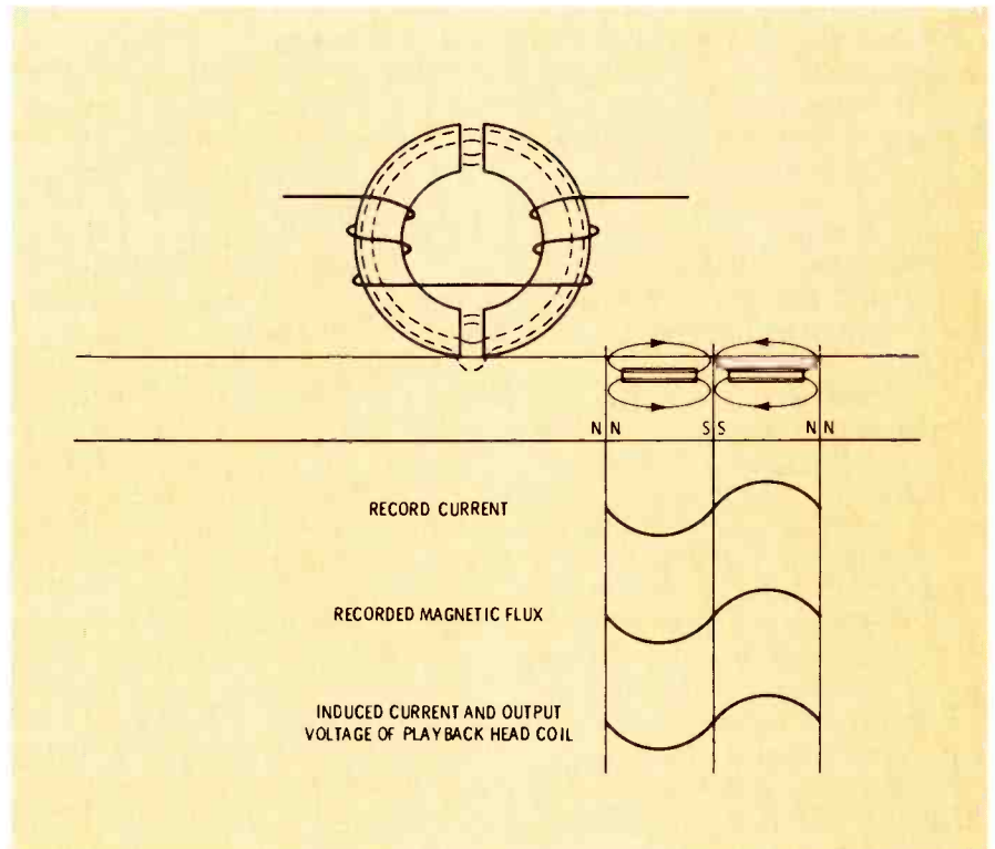
Fig. 3 It's impossible to record a sine wave that occupies less space than the width of the gap. That's called the "extinction" frequency.
