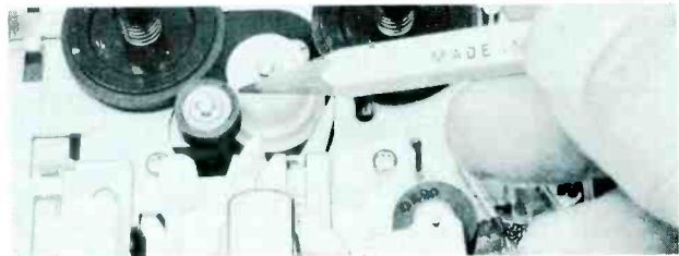
Step 15. Rewind and Fast Forward usually are driven from the same flywheel idler. The entire fast-forward drive train, plus an extra idler, comes into use when you press the Rewind button. The rewind idler, the added one, presses against both fast-forward idler and supply spindle, spinning the spindle rapidly in reverse. Usually, you'll find no torque adjustment here. If rewind becomes erratic or too slow, you hunt for weak or unhooked springs or binding idlers.
